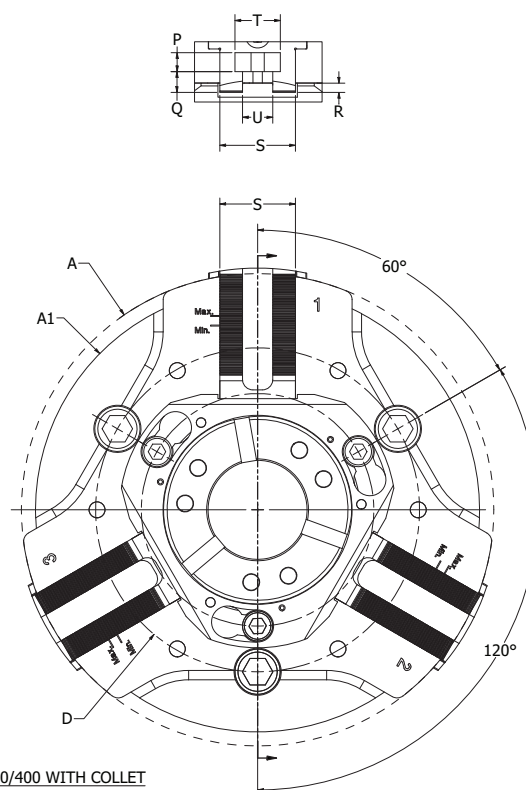
MTC-200/250/320/350/400 WITH COLLET
