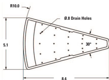
Bin Dimensions
