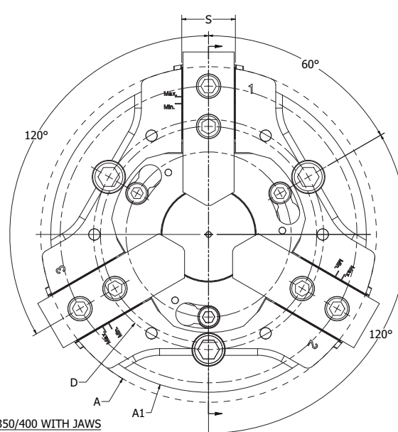
MTC-200/250/320/350/400 WITH JAWS
