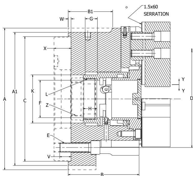
MTC-200/250/320/350/400 WITH JAWS
