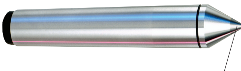
Type 2 Standard Dead Center with carbide tip add "2" to part number below.
